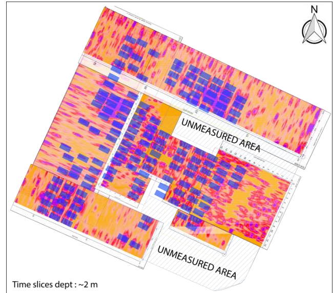
Figure 7. Marking of possible findings (anomalies) on GPR results (blue areas show possible war graves).
